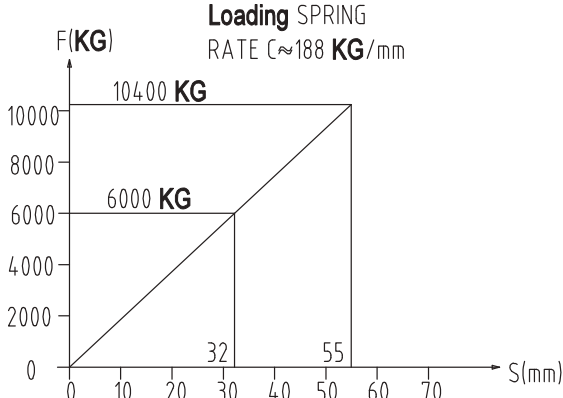
LOAD DEFLECTION DIAGRAM
